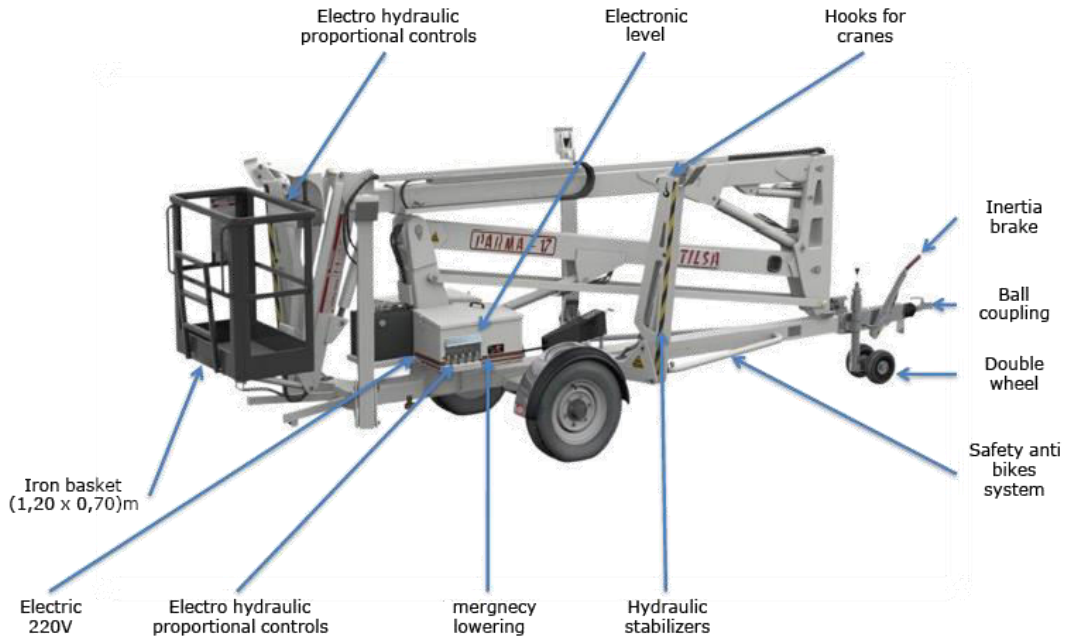
A Standard Parma 17 unit
