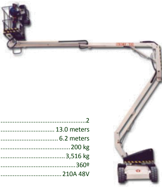
A Parma 13E unit with optional accessories attached to it
